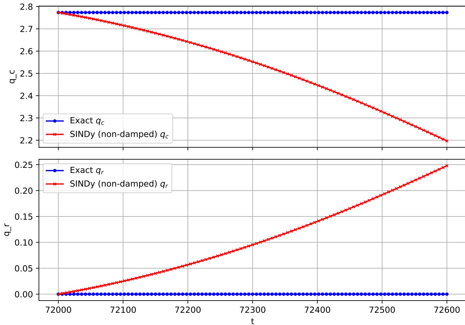
Trajectory 2419 (non-damped)
