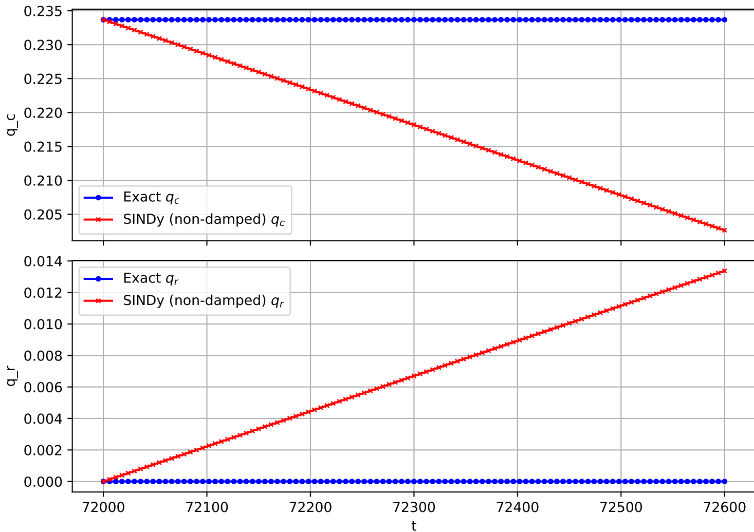
Trajectory 2425 (non-damped)
