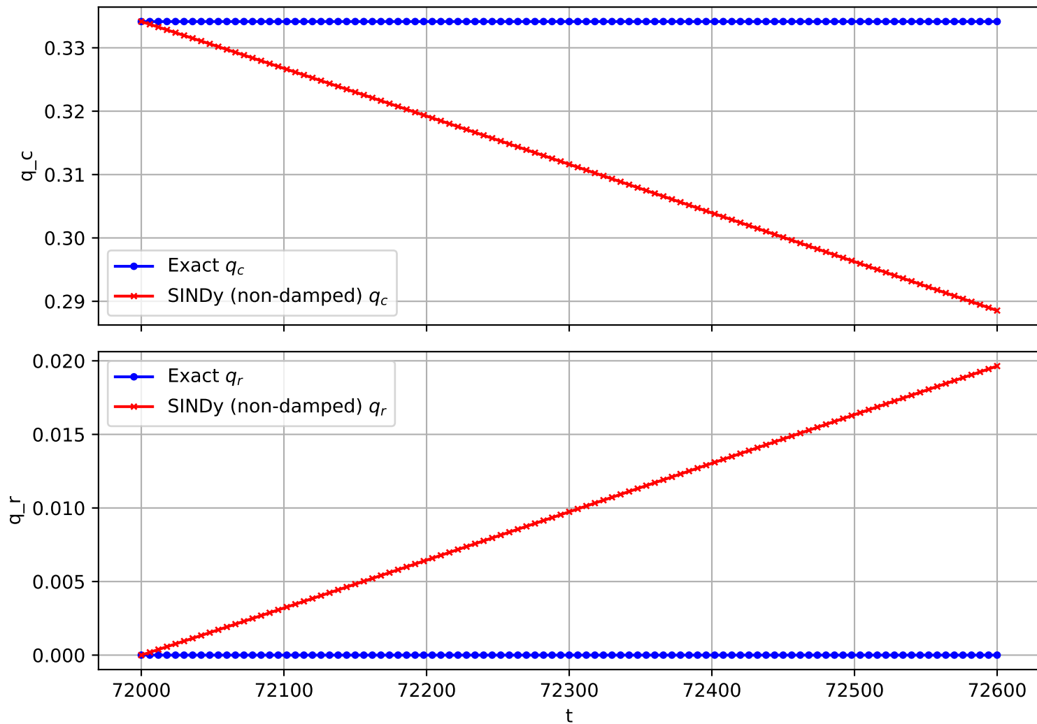
Trajectory 2426 (non-damped)
