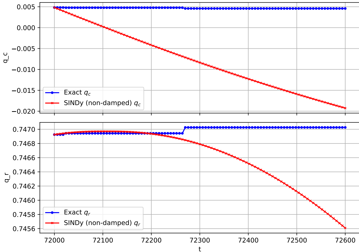
Trajectory 2434 (non-damped)
