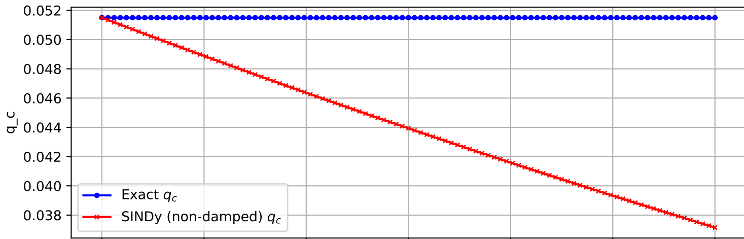
Trajectory 2449 (non-damped)
