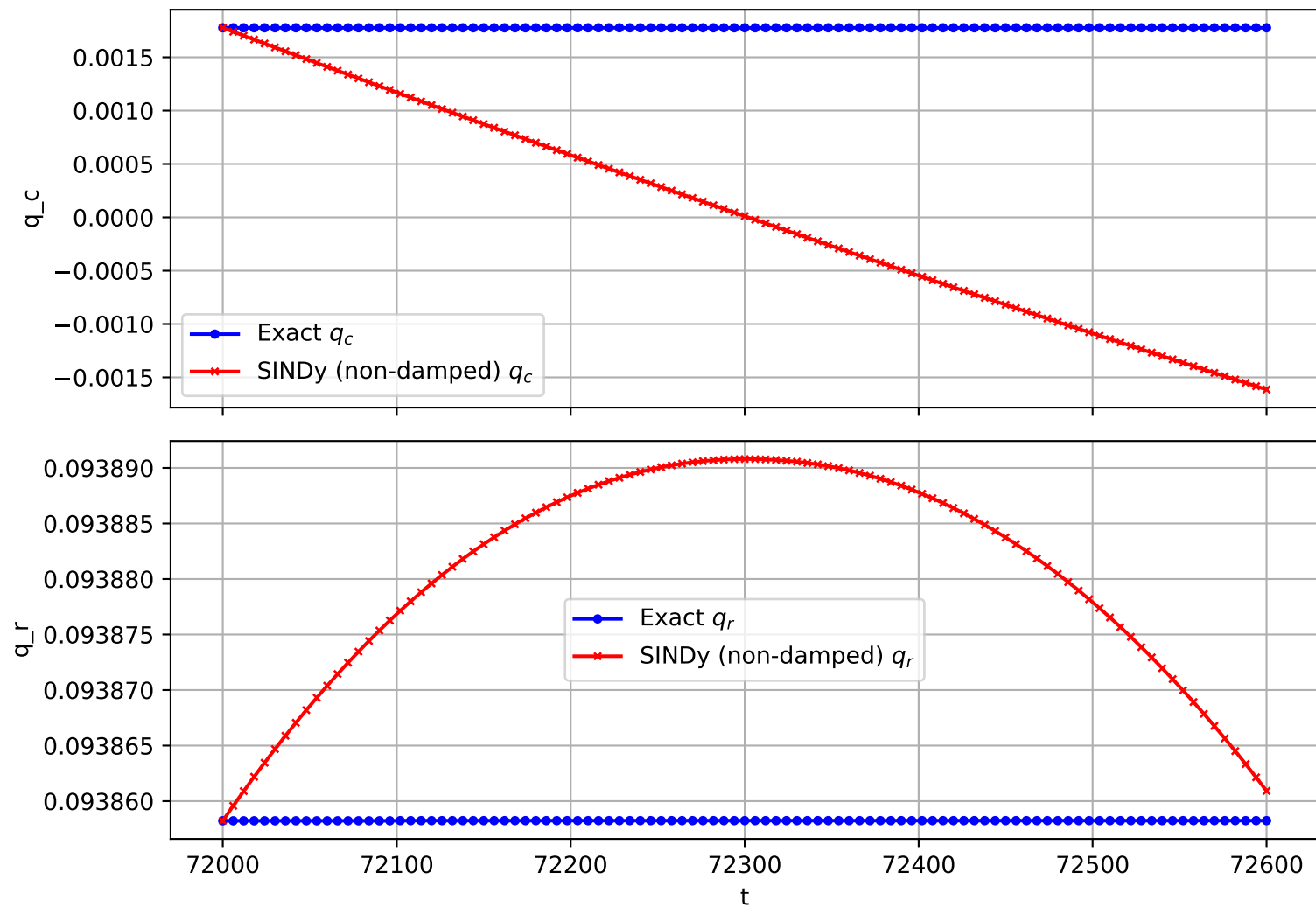
Trajectory 2451 (non-damped)
