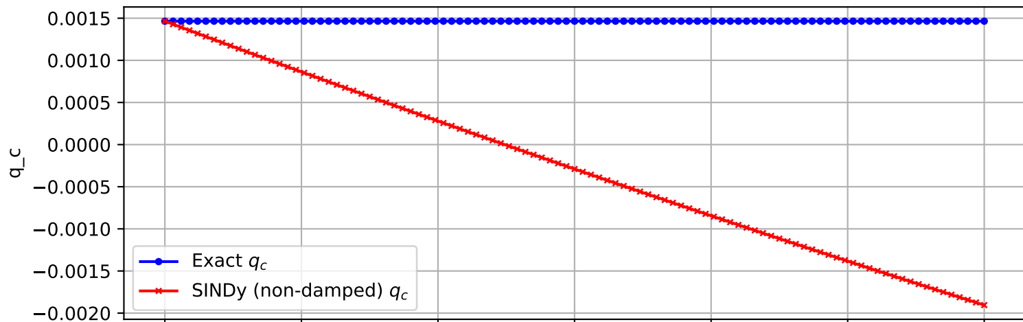
Trajectory 2454 (non-damped)
