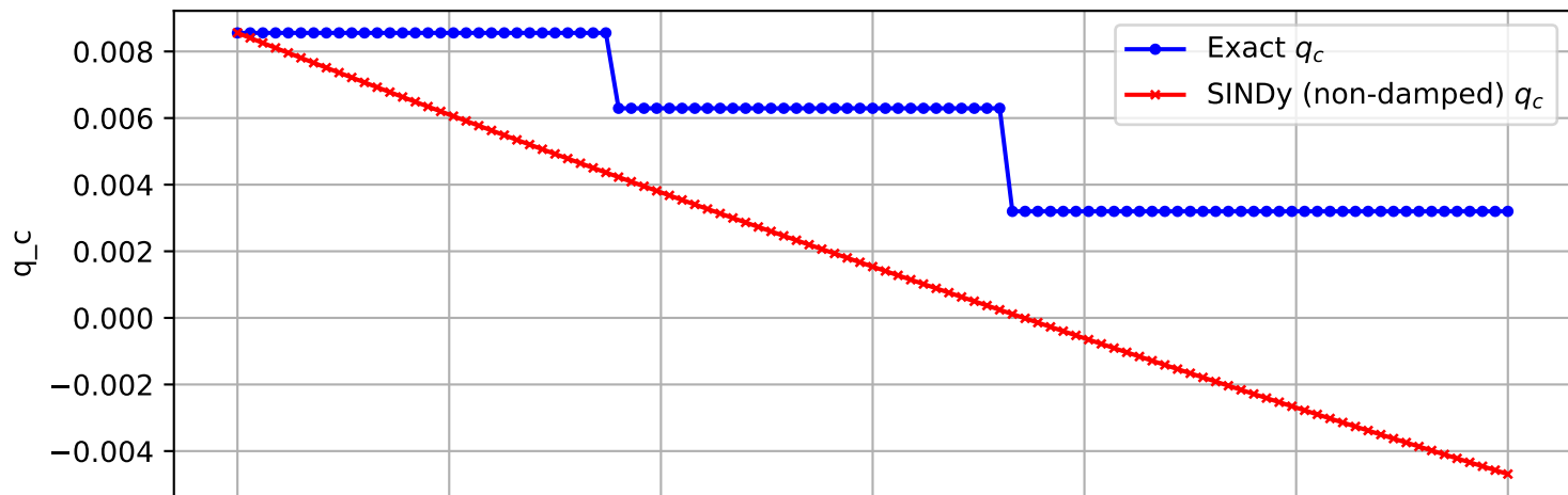
Trajectory 2459 (non-damped)
