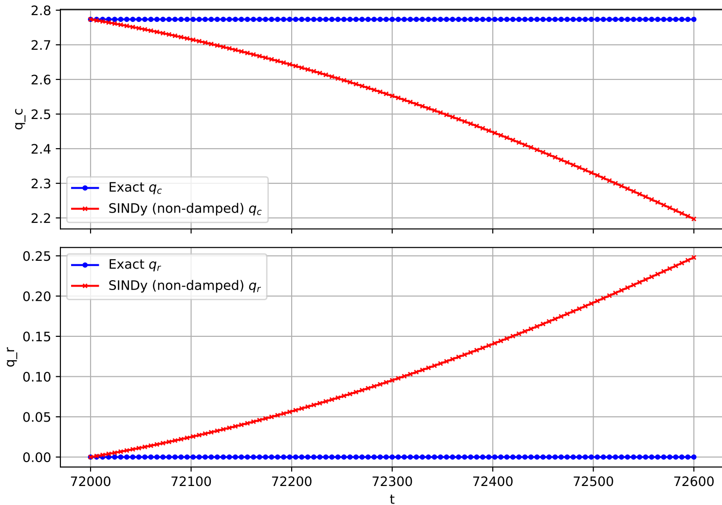
Trajectory 2486 (non-damped)
