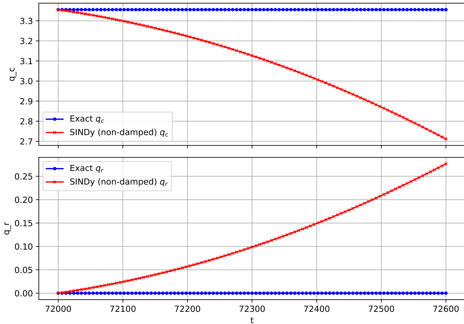
Trajectory 2490 (non-damped)
