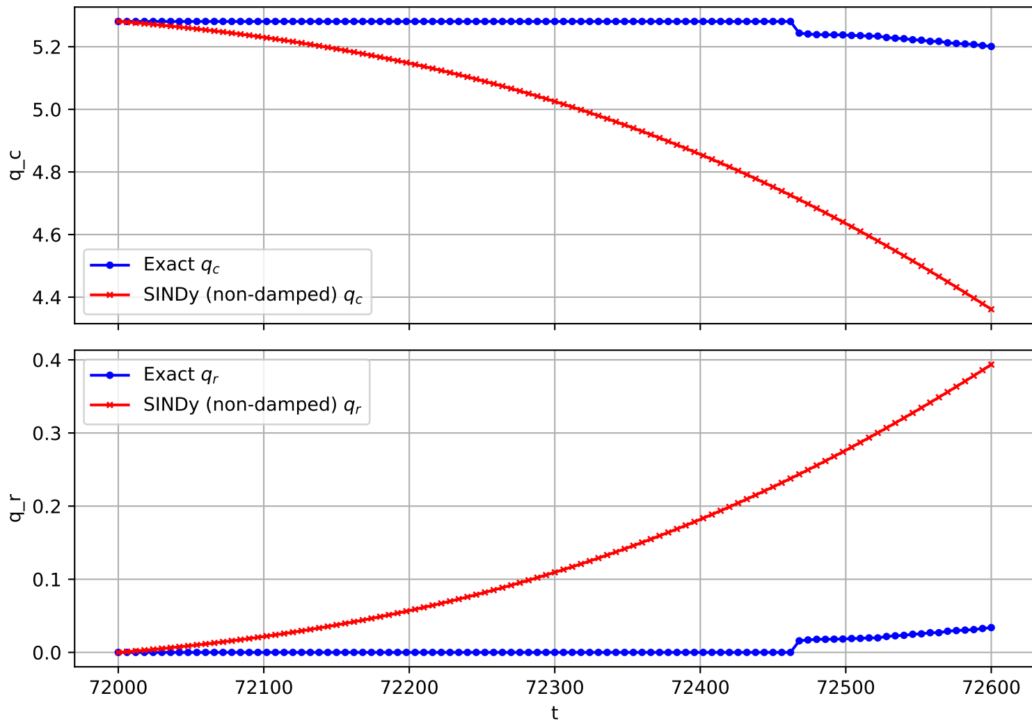
Trajectory 2492 (non-damped)
