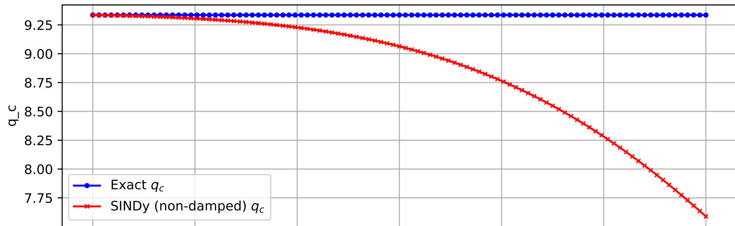
Trajectory 2494 (non-damped)
