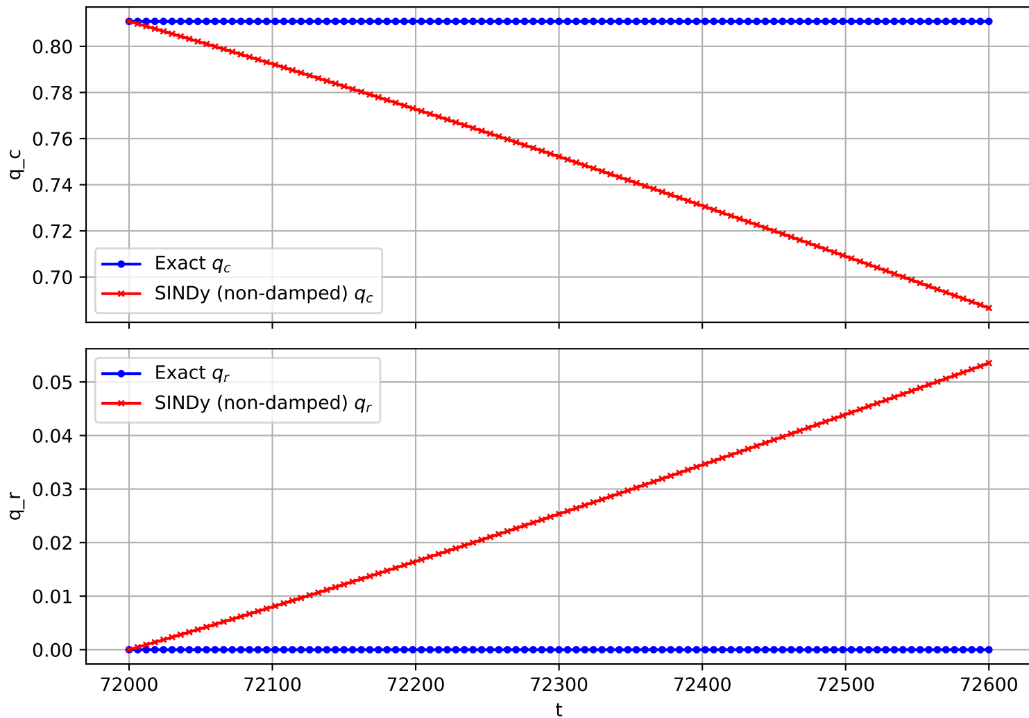
Trajectory 2499 (non-damped)
