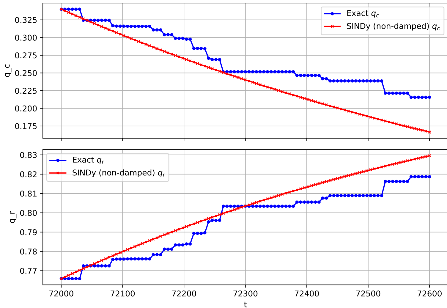
Trajectory 2503 (non-damped)
