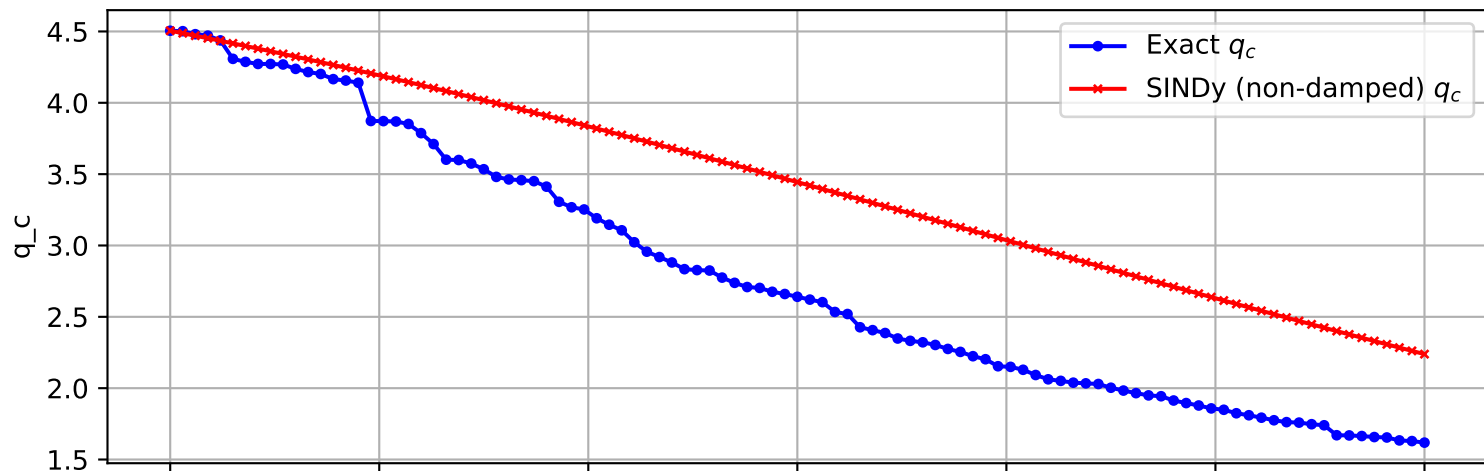
Trajectory 2504 (non-damped)
