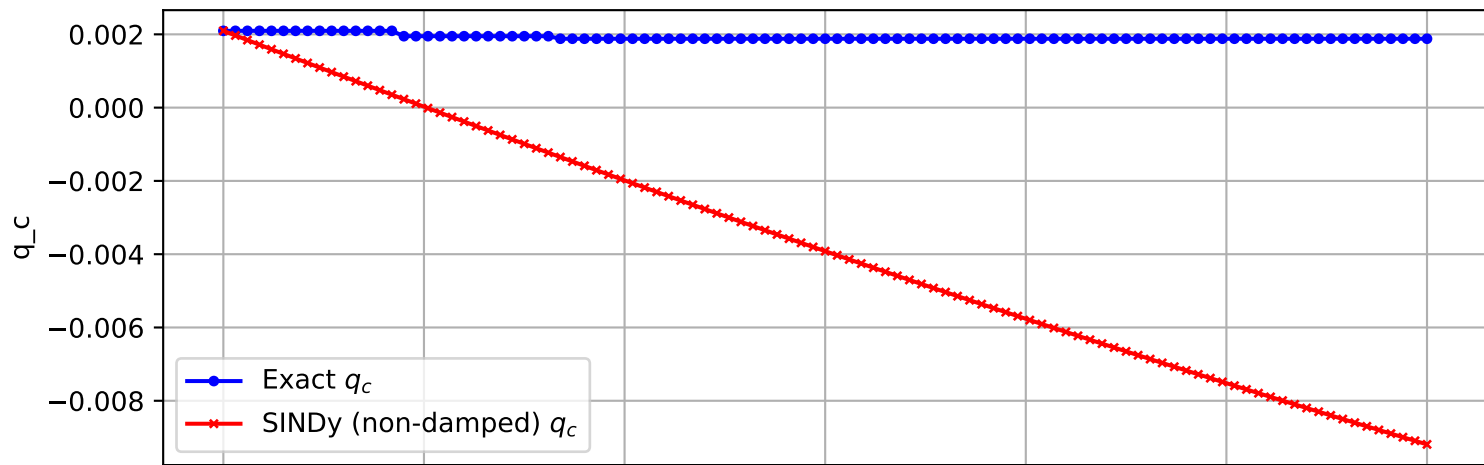
Trajectory 2511 (non-damped)
