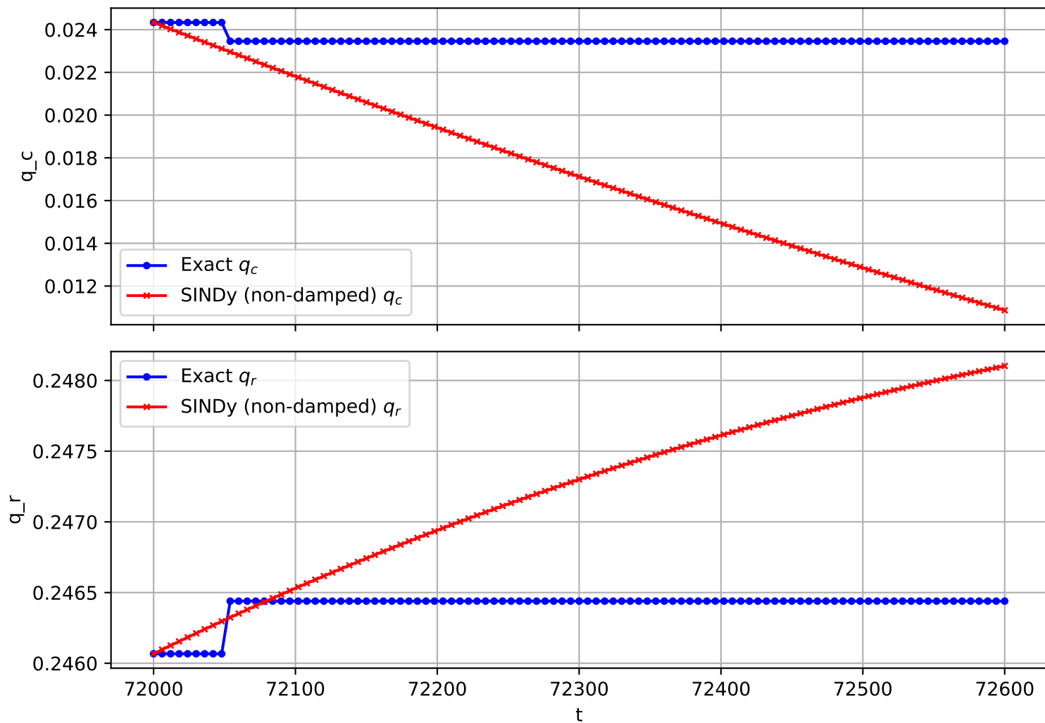
Trajectory 2513 (non-damped)
