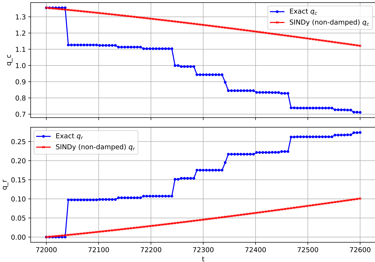
Trajectory 2515 (non-damped)
