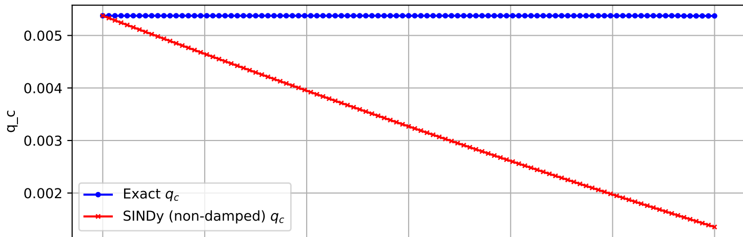
Trajectory 2518 (non-damped)
