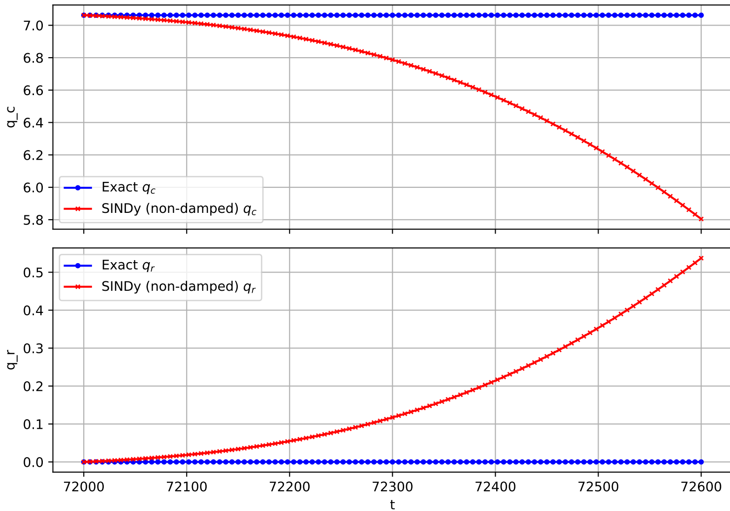
Trajectory 2523 (non-damped)
