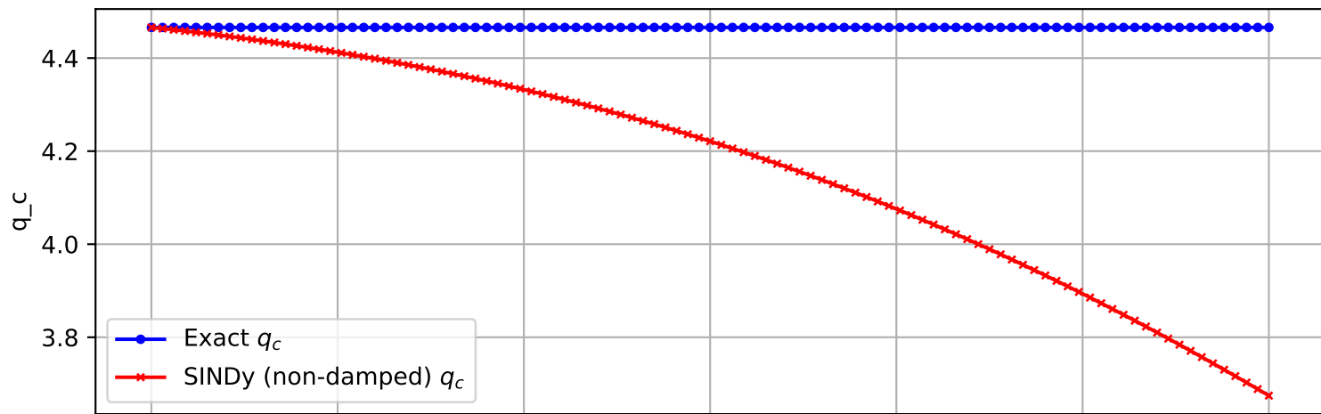
Trajectory 2526 (non-damped)
