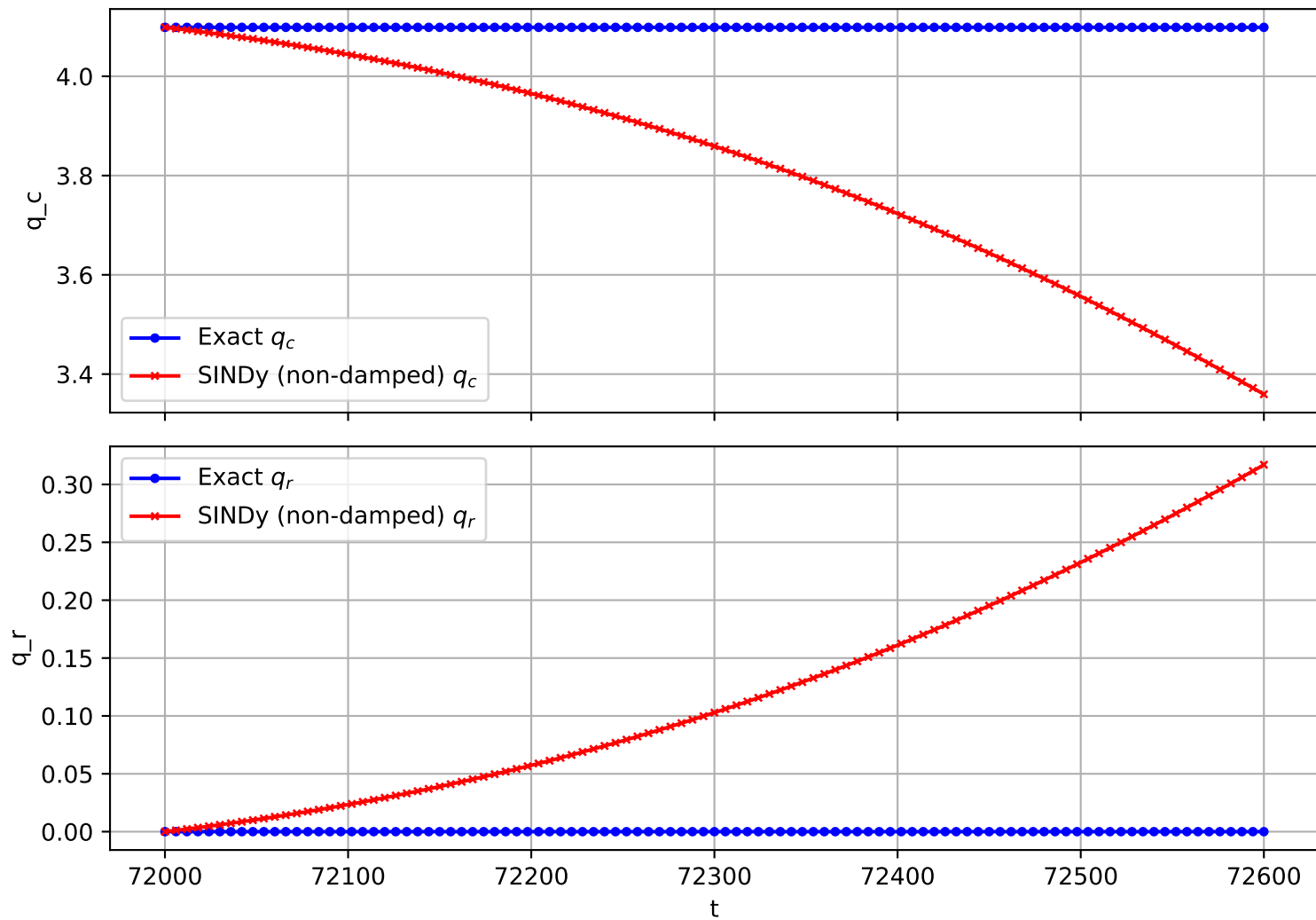
Trajectory 2533 (non-damped)
