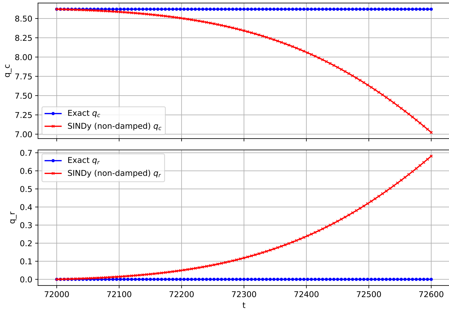
Trajectory 2534 (non-damped)
