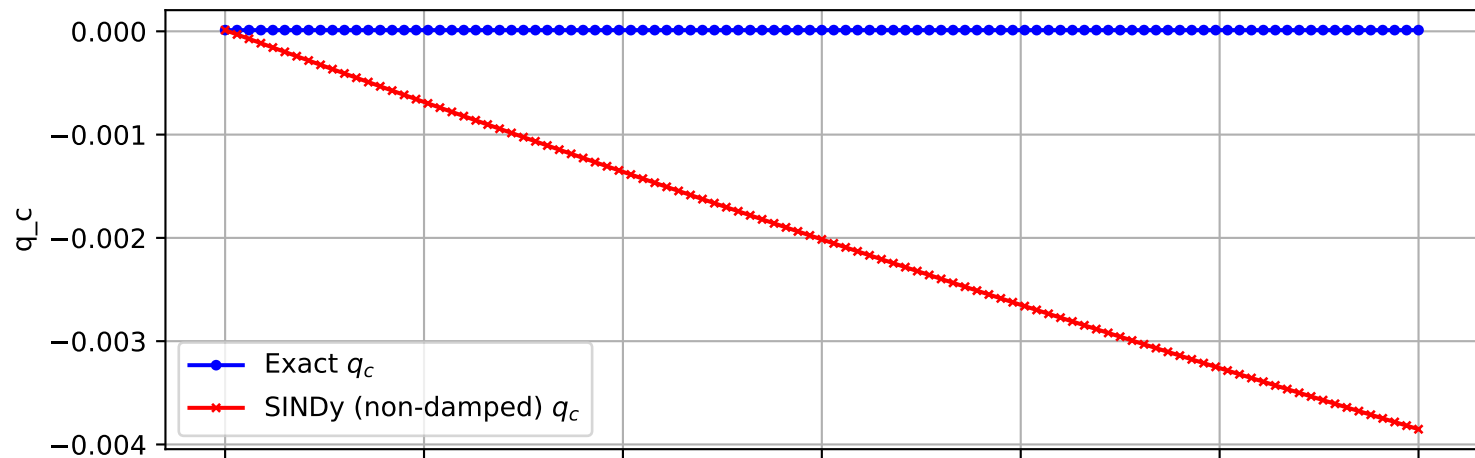
Trajectory 2538 (non-damped)
