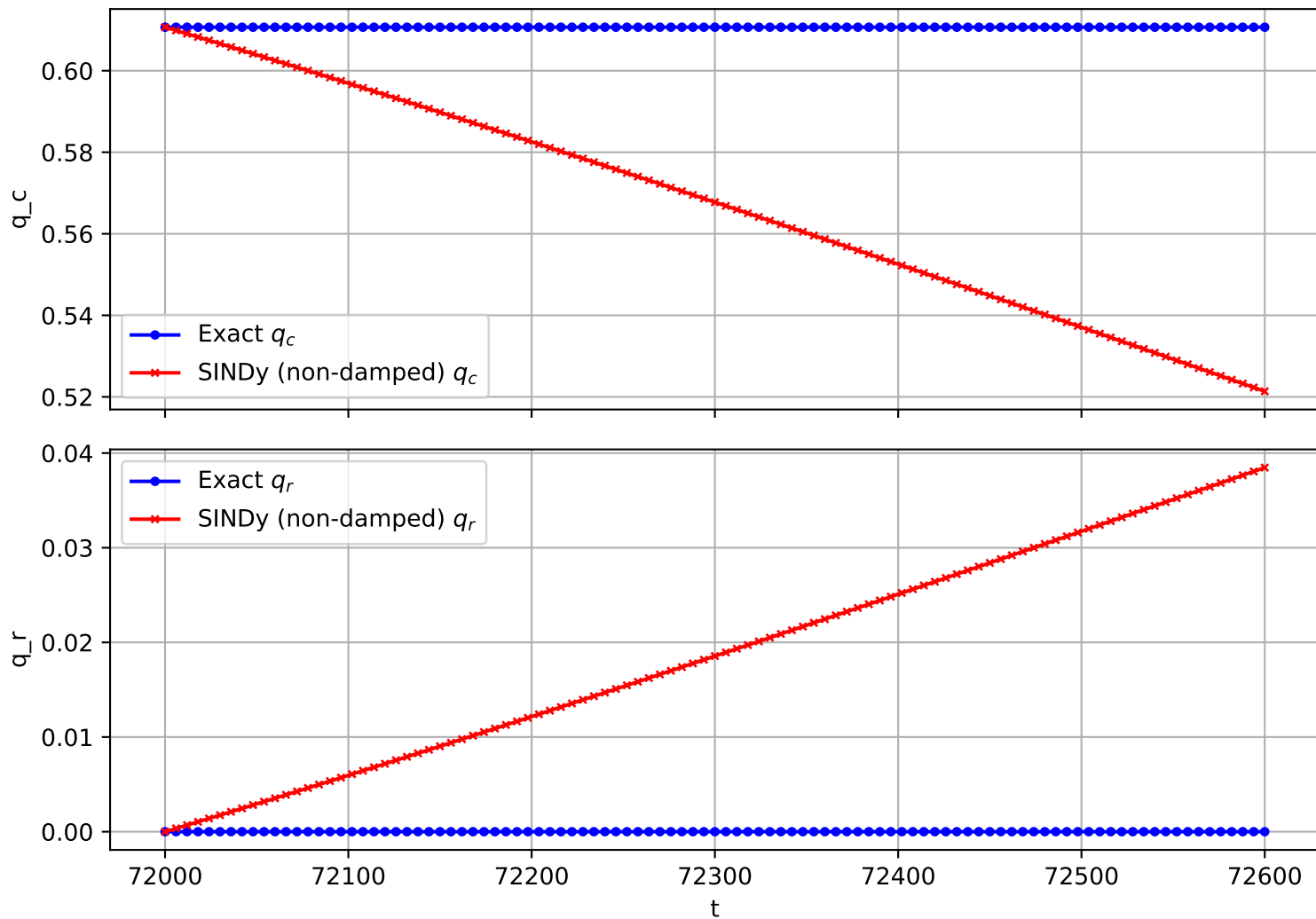
Trajectory 2545 (non-damped)
