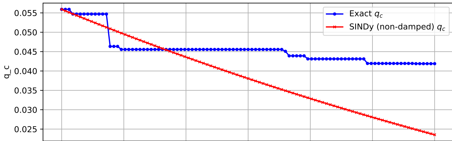
Trajectory 2549 (non-damped)
