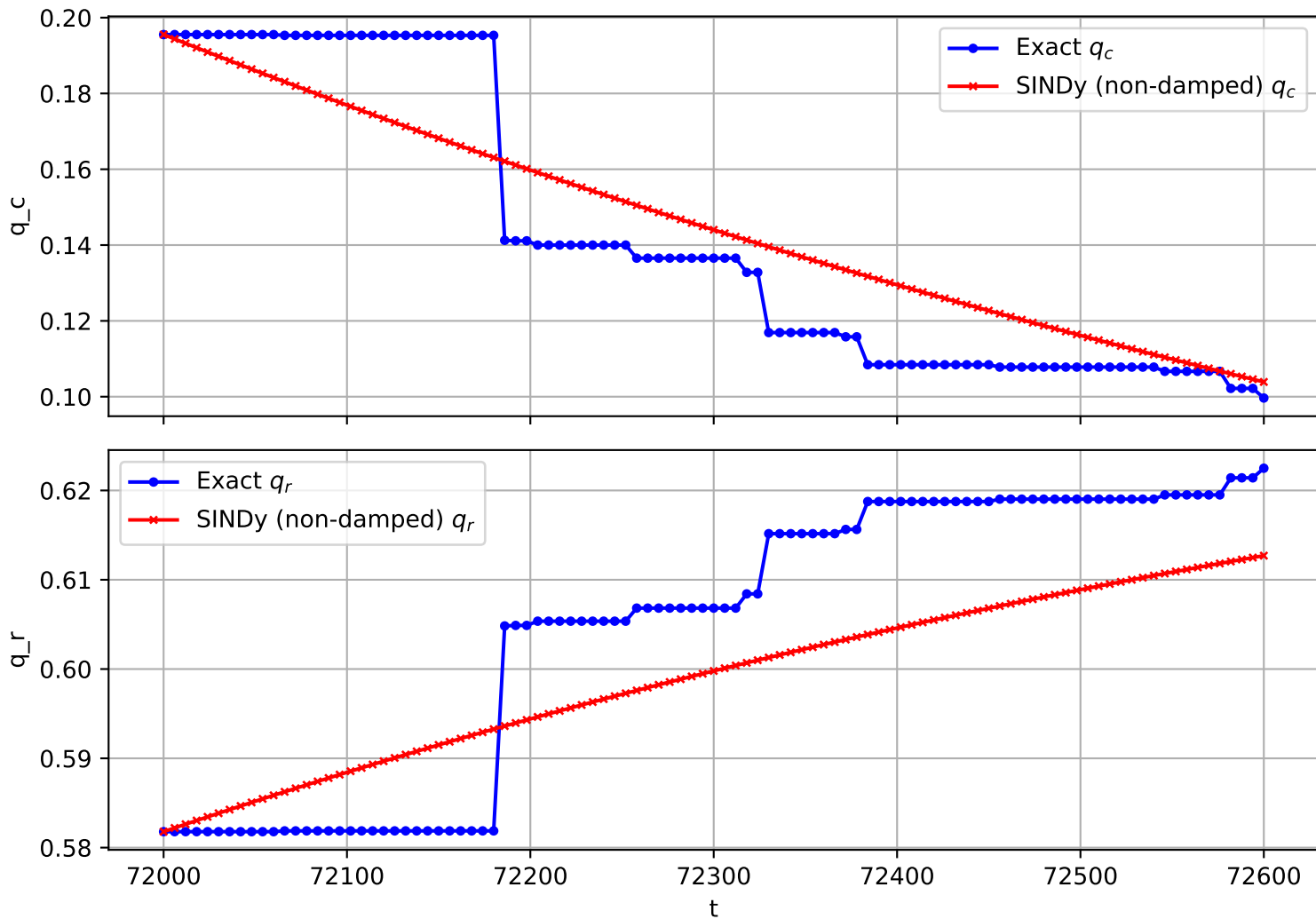
Trajectory 2550 (non-damped)
