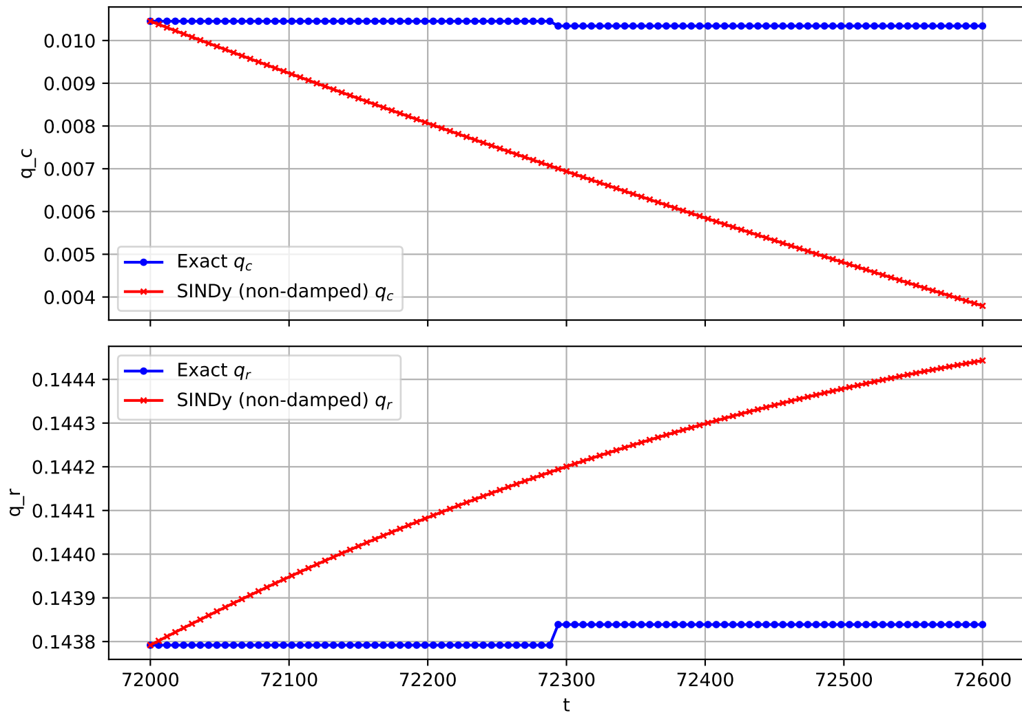
Trajectory 2554 (non-damped)
