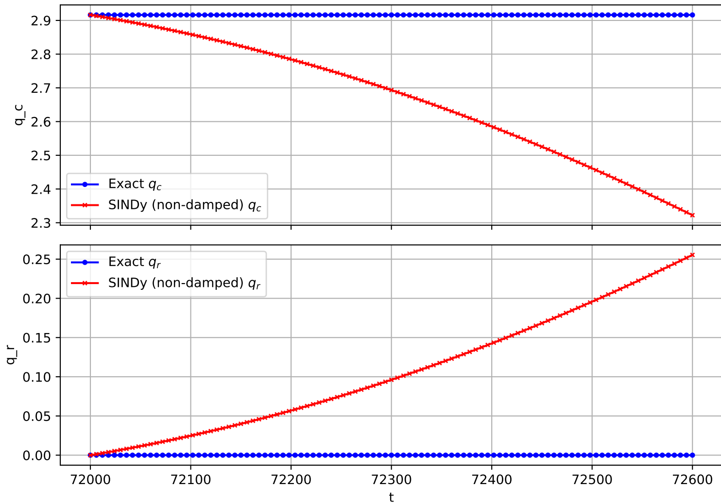
Trajectory 2559 (non-damped)
