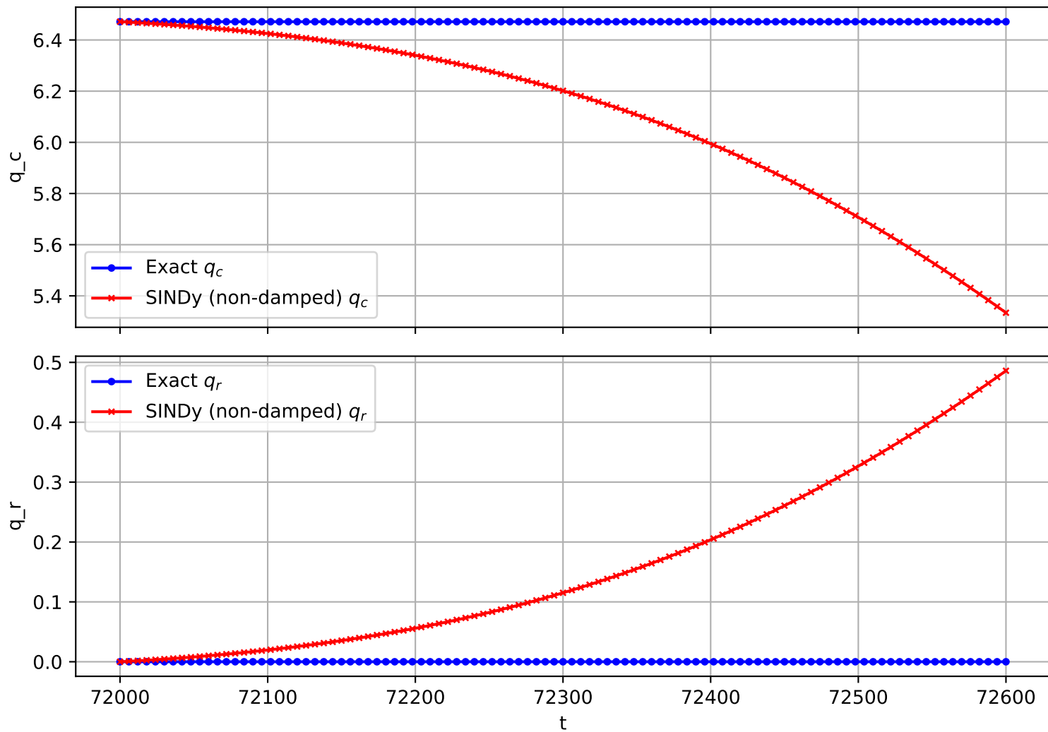
Trajectory 2563 (non-damped)
