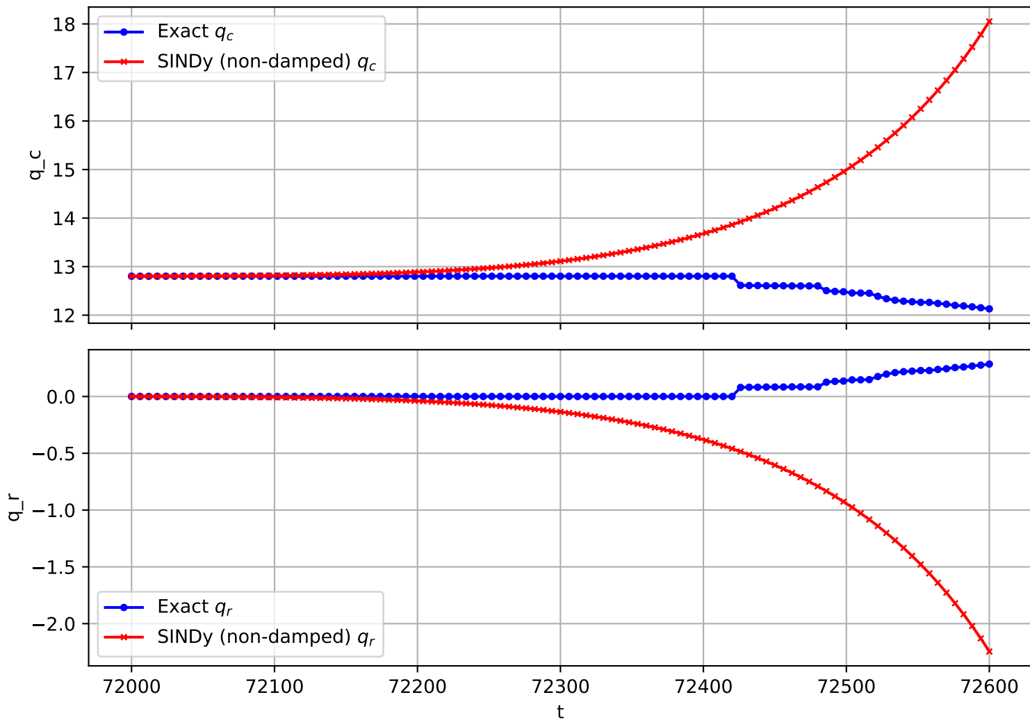
Trajectory 2570 (non-damped)
