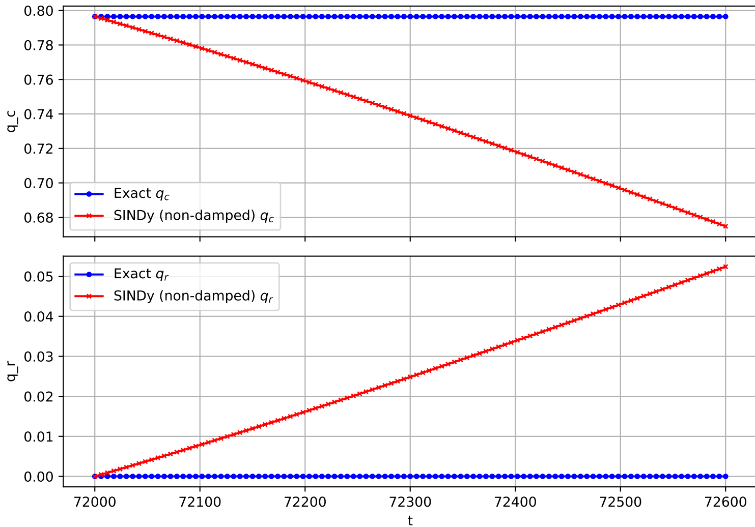
Trajectory 2572 (non-damped)
