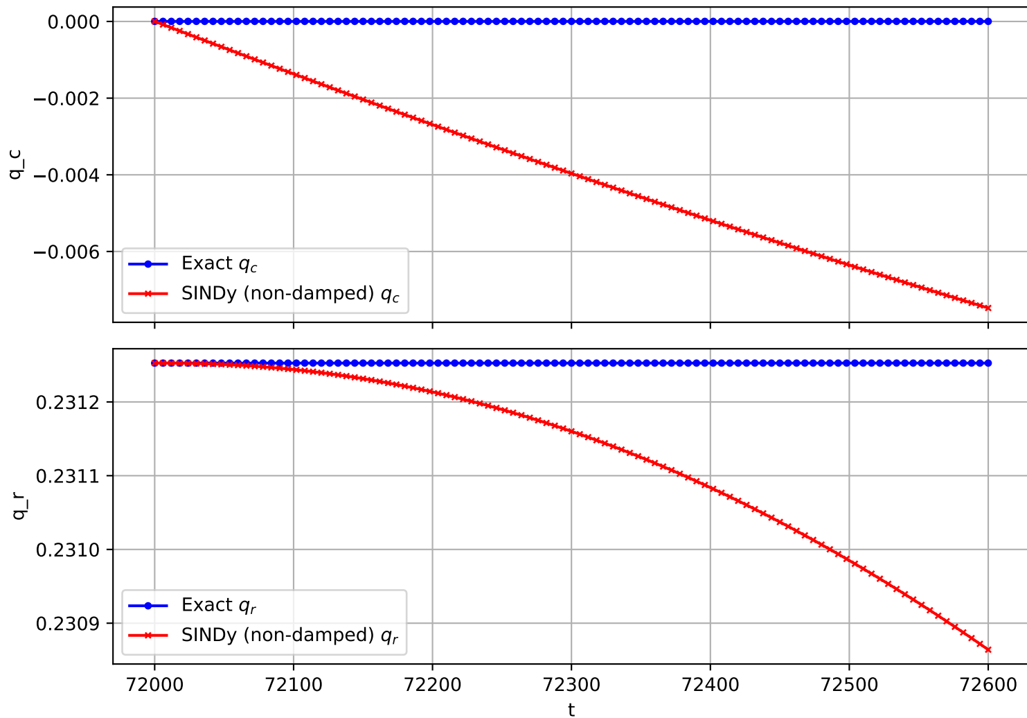
Trajectory 2576 (non-damped)
