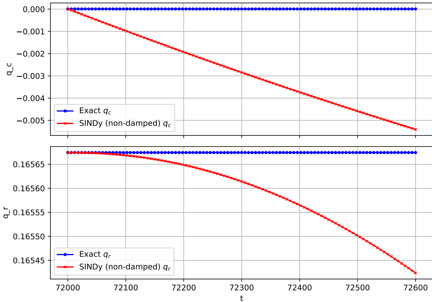
Trajectory 2579 (non-damped)
