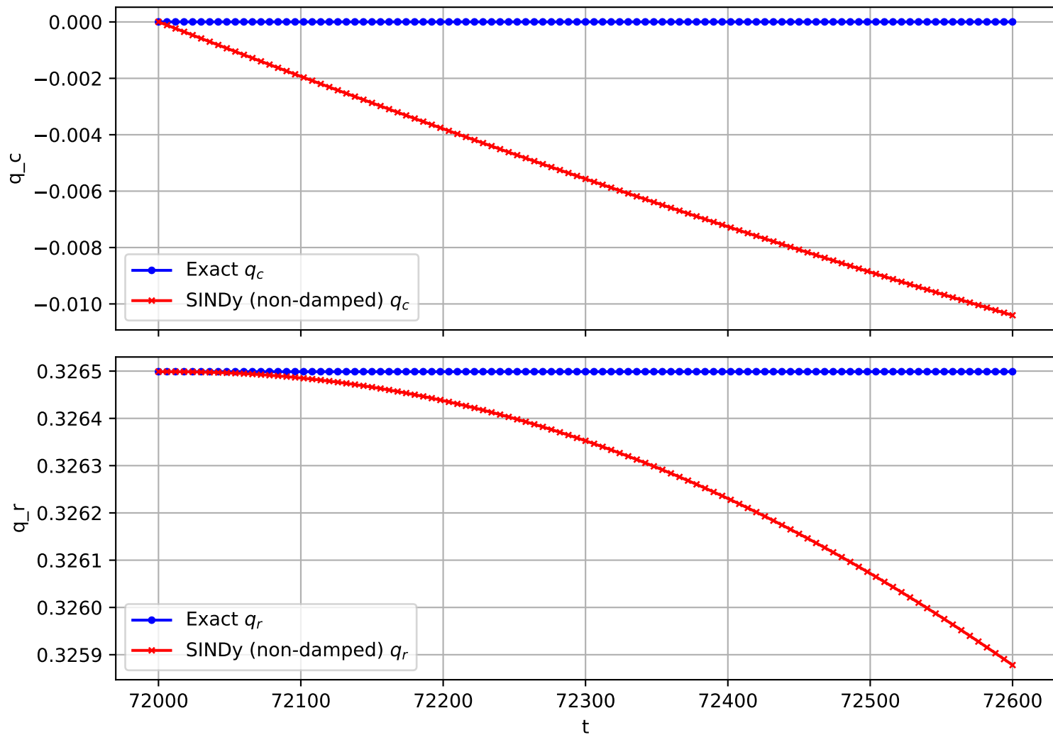
Trajectory 2583 (non-damped)
