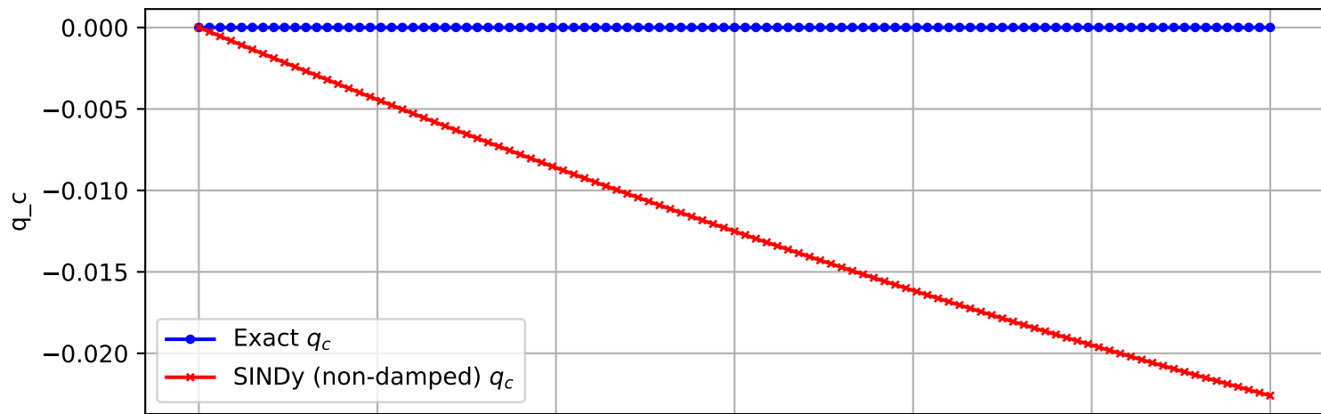
Trajectory 2599 (non-damped)
