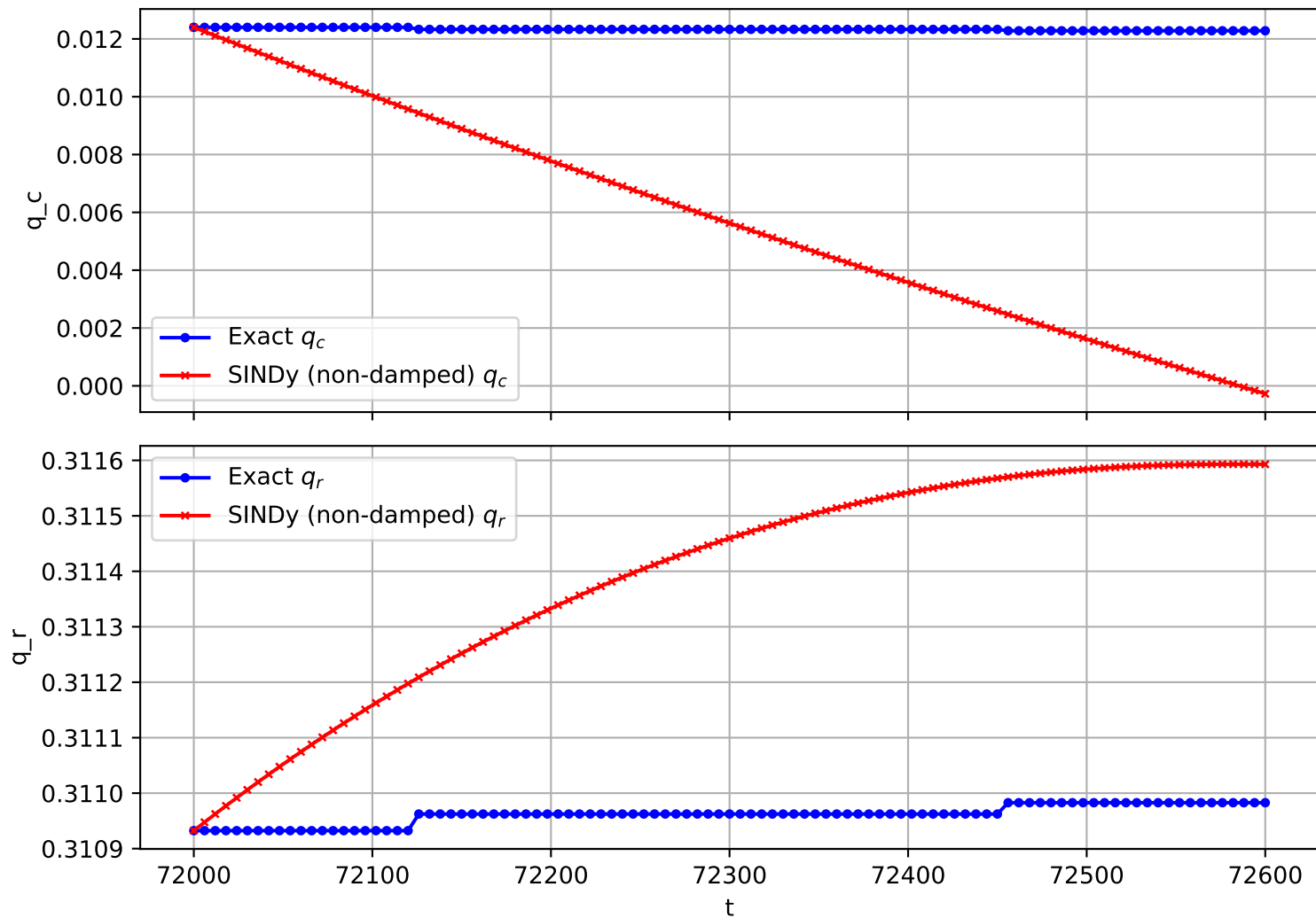
Trajectory 2608 (non-damped)
