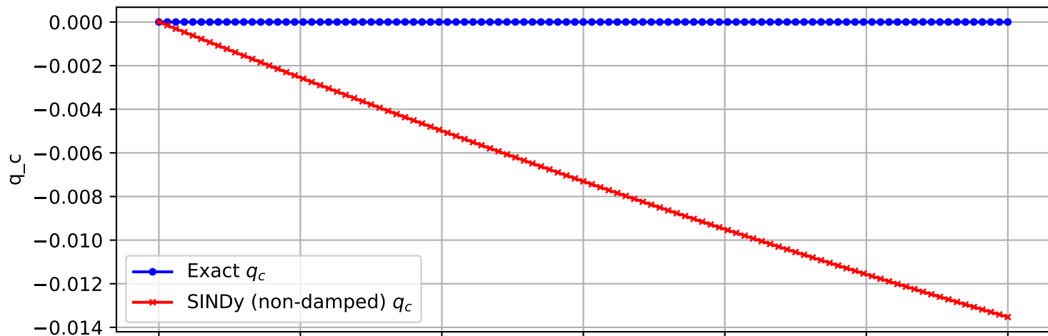
Trajectory 2611 (non-damped)
