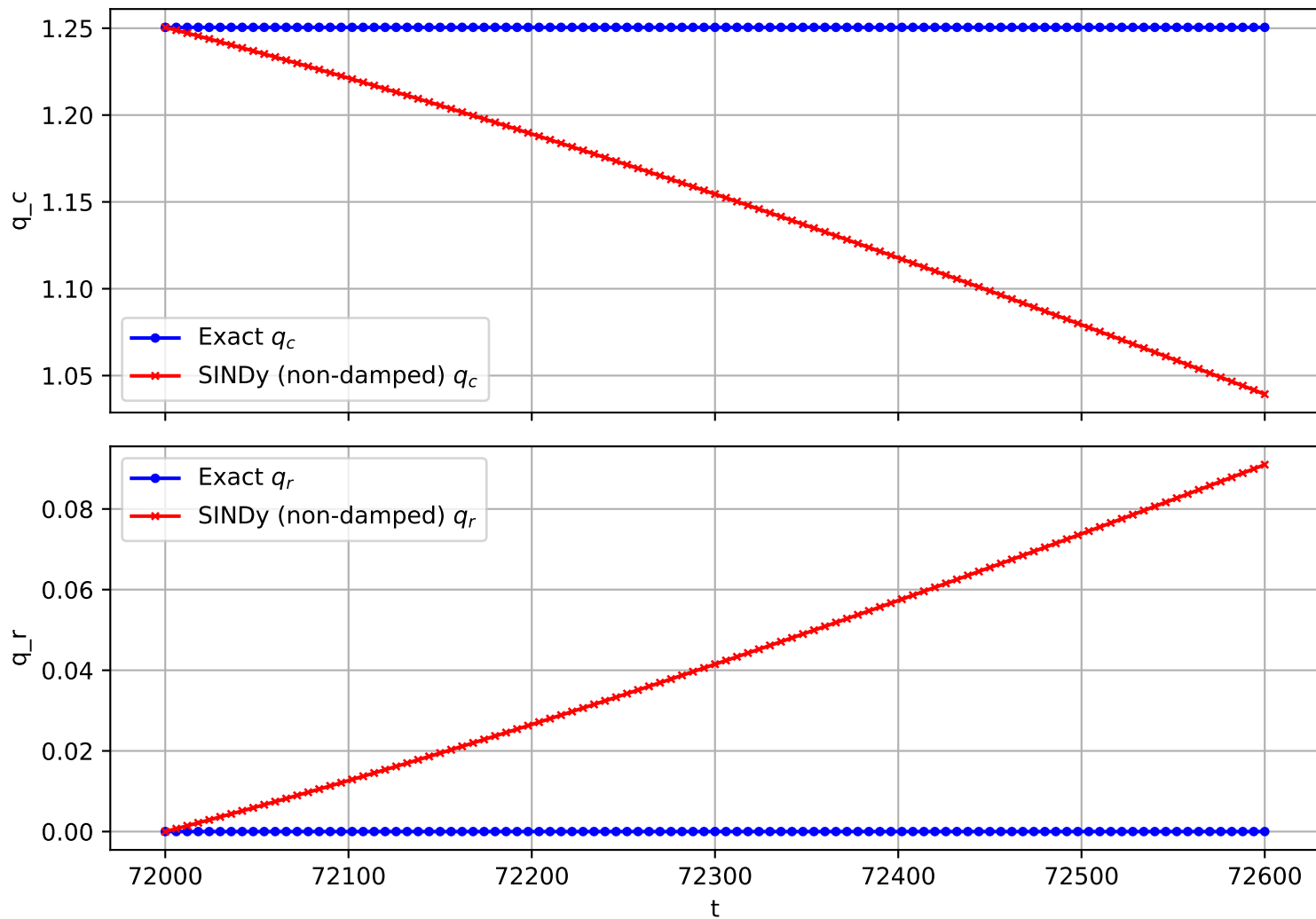
Trajectory 262 (non-damped)
