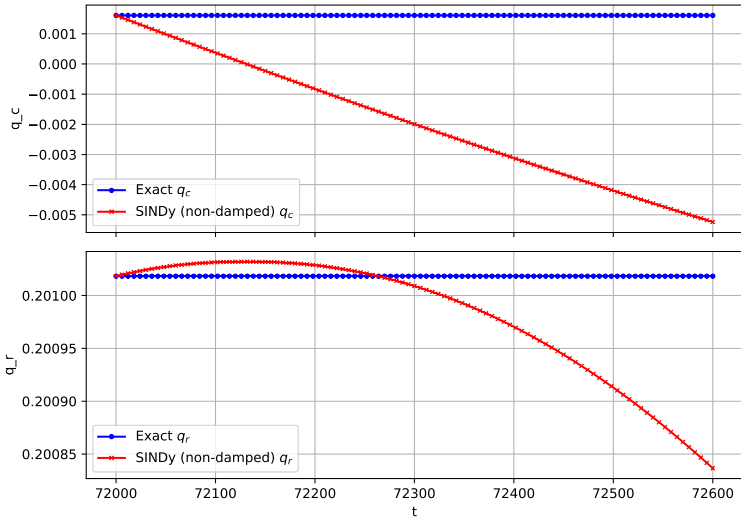
Trajectory 2621 (non-damped)
