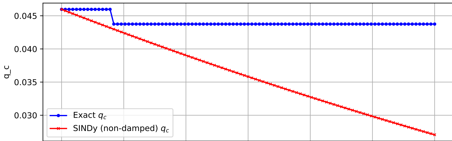
Trajectory 2622 (non-damped)
