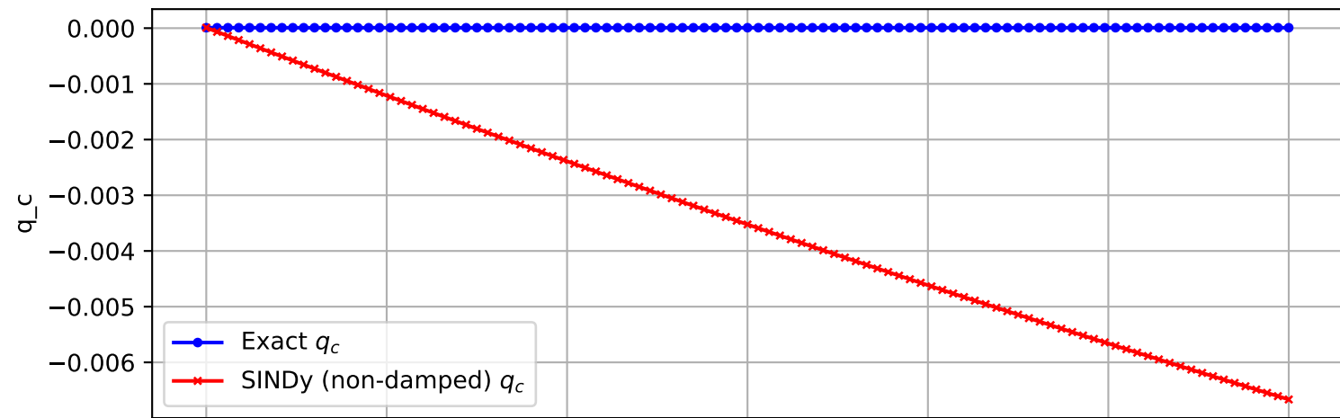
Trajectory 2625 (non-damped)
