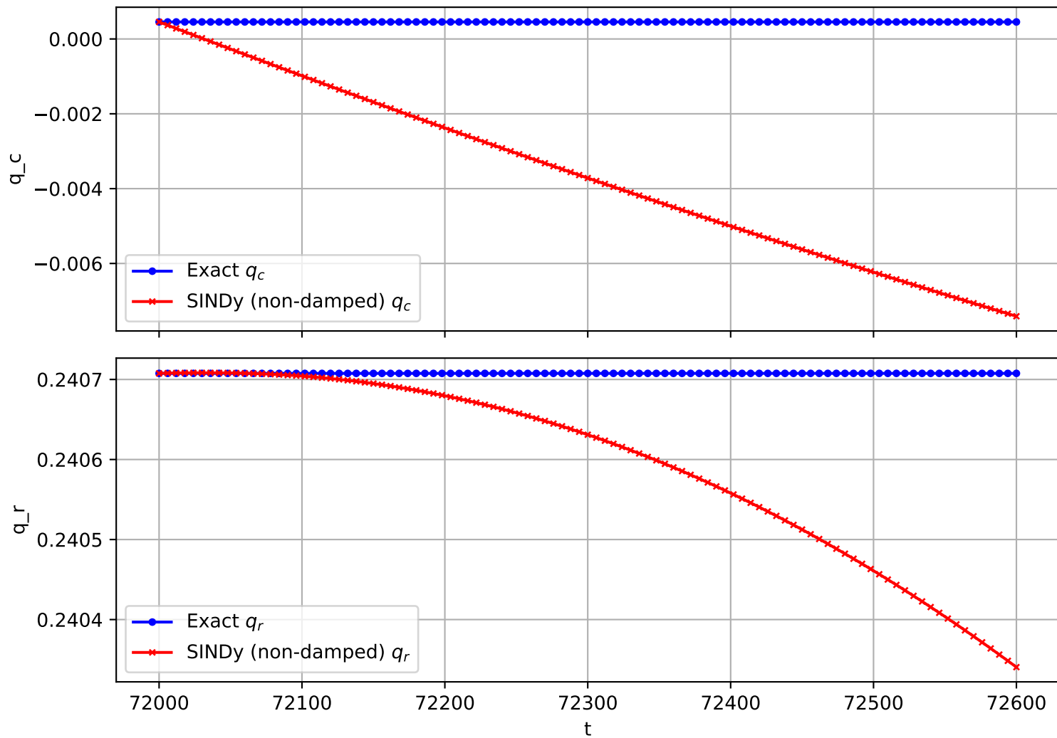
Trajectory 2643 (non-damped)
