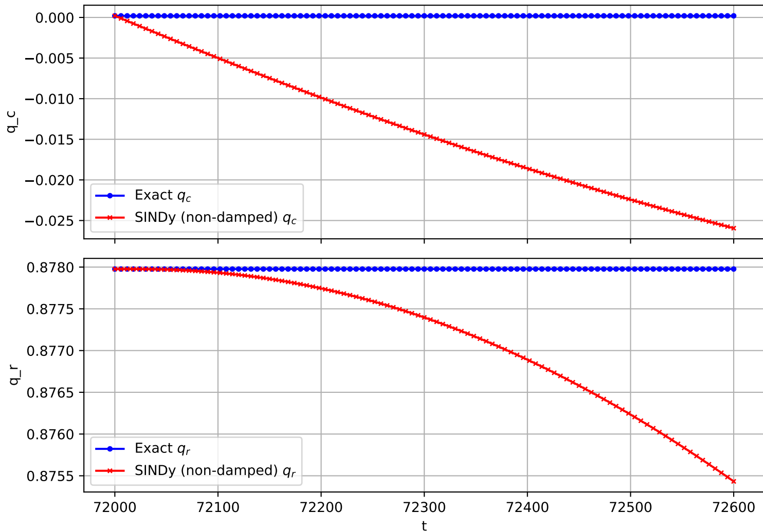
Trajectory 2650 (non-damped)
