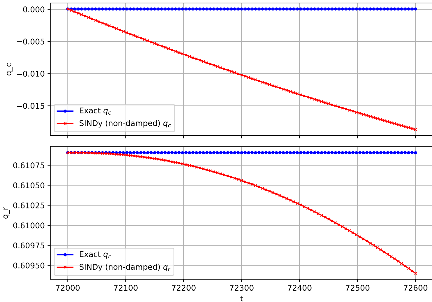
Trajectory 2651 (non-damped)
