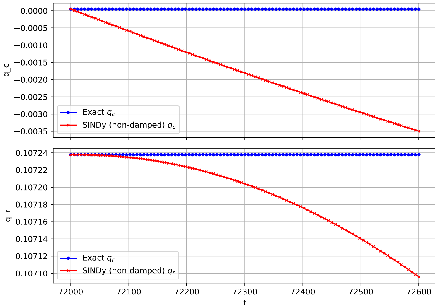
Trajectory 2653 (non-damped)
