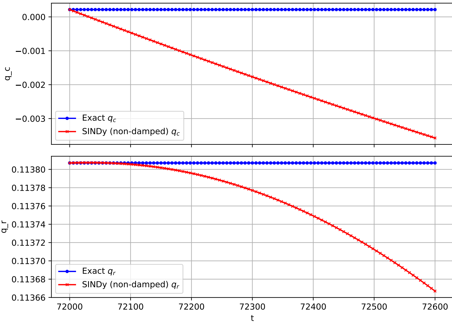
Trajectory 2654 (non-damped)
