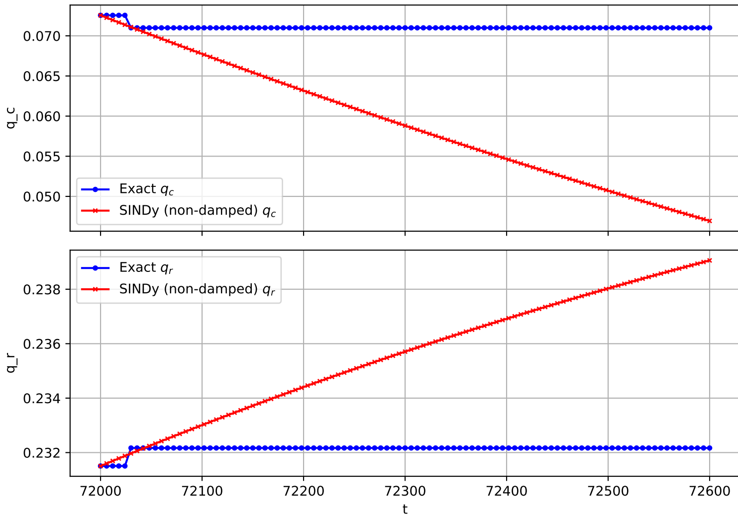
Trajectory 2658 (non-damped)
