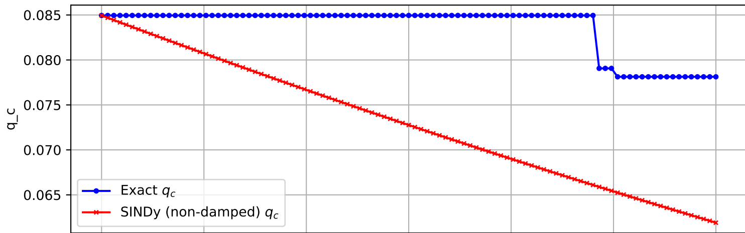
Trajectory 2661 (non-damped)
