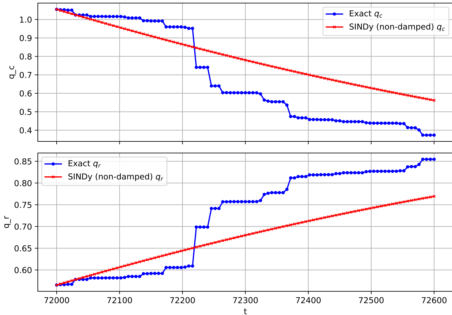
Trajectory 2663 (non-damped)
